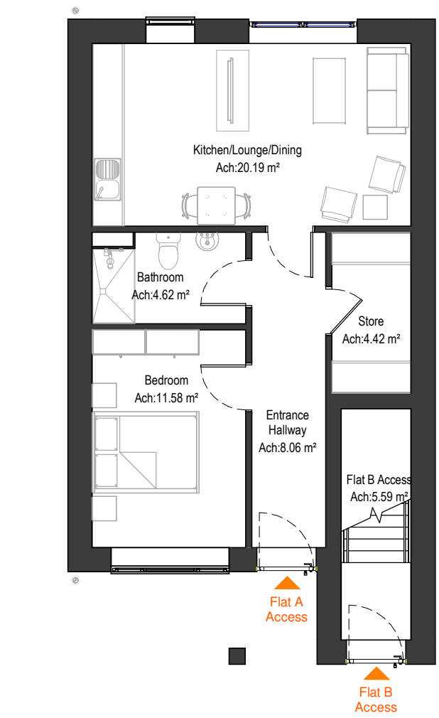
GF_F1 Ground Floor Plan 1 : 100
